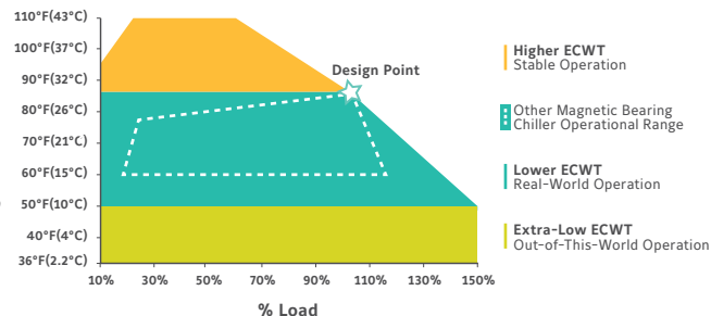
YMC 2 Operating Envelope
