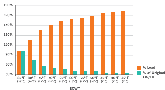
Chiller Max Capacities and kW/TR at Reduced ECWT
