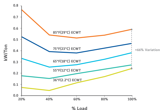
YMC 2 Chiller Performance Below 0.1 kW/Ton
