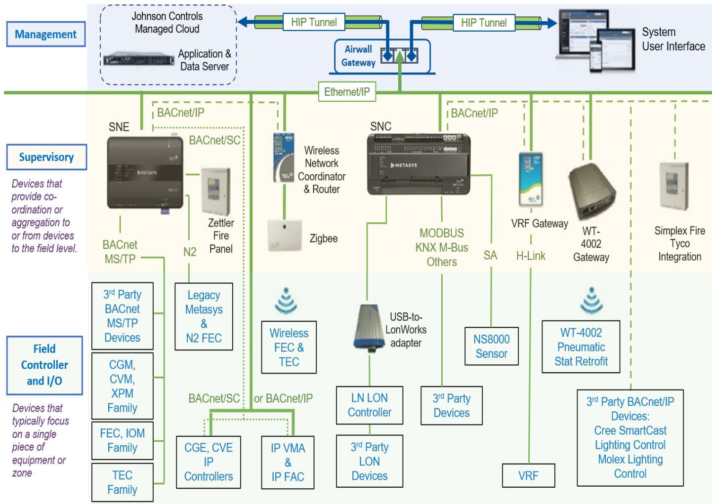
Figure 1.1.1.2: Managed Metasys system (ADX servers only) architecture example
