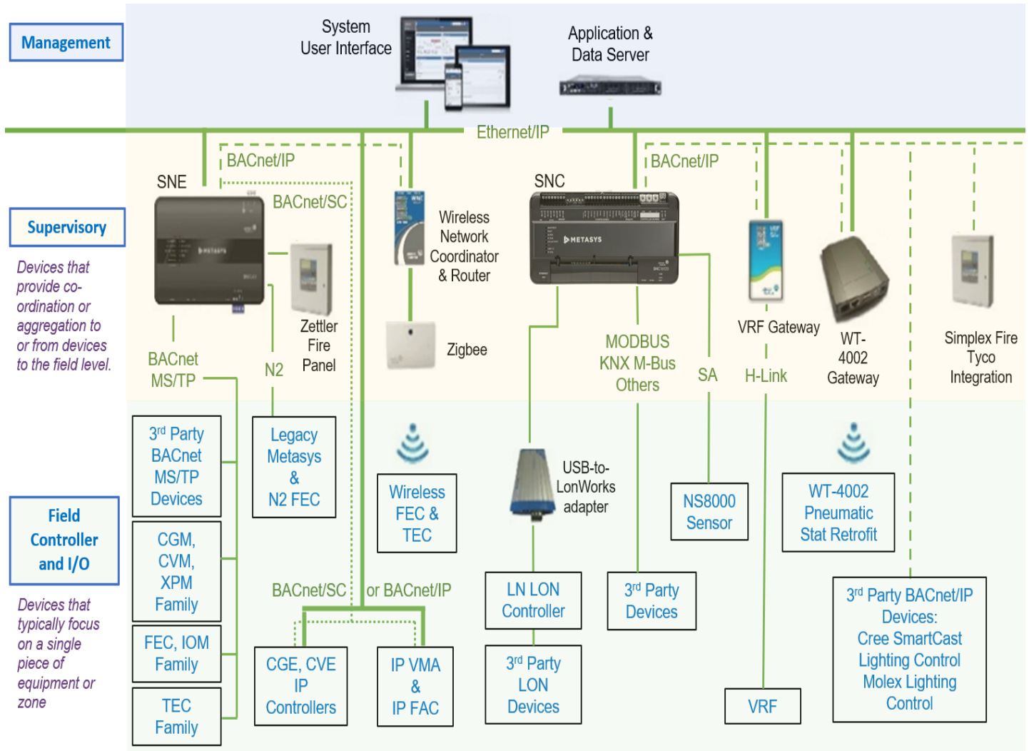
Figure 1.1.1.1: Metasys system on premises architecture example
