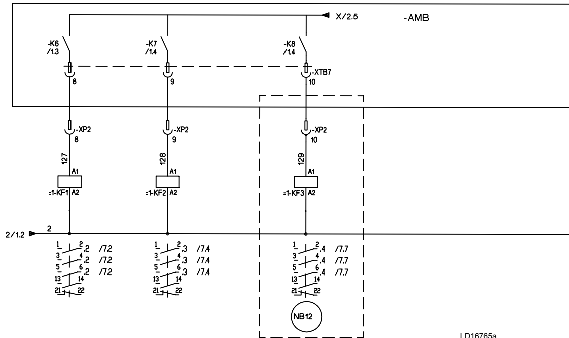
FIGURE 14 - FAN WIRING, STANDARD LOW SOUND OR ULTRA QUIET, YLAA0070 - YLAA0516
