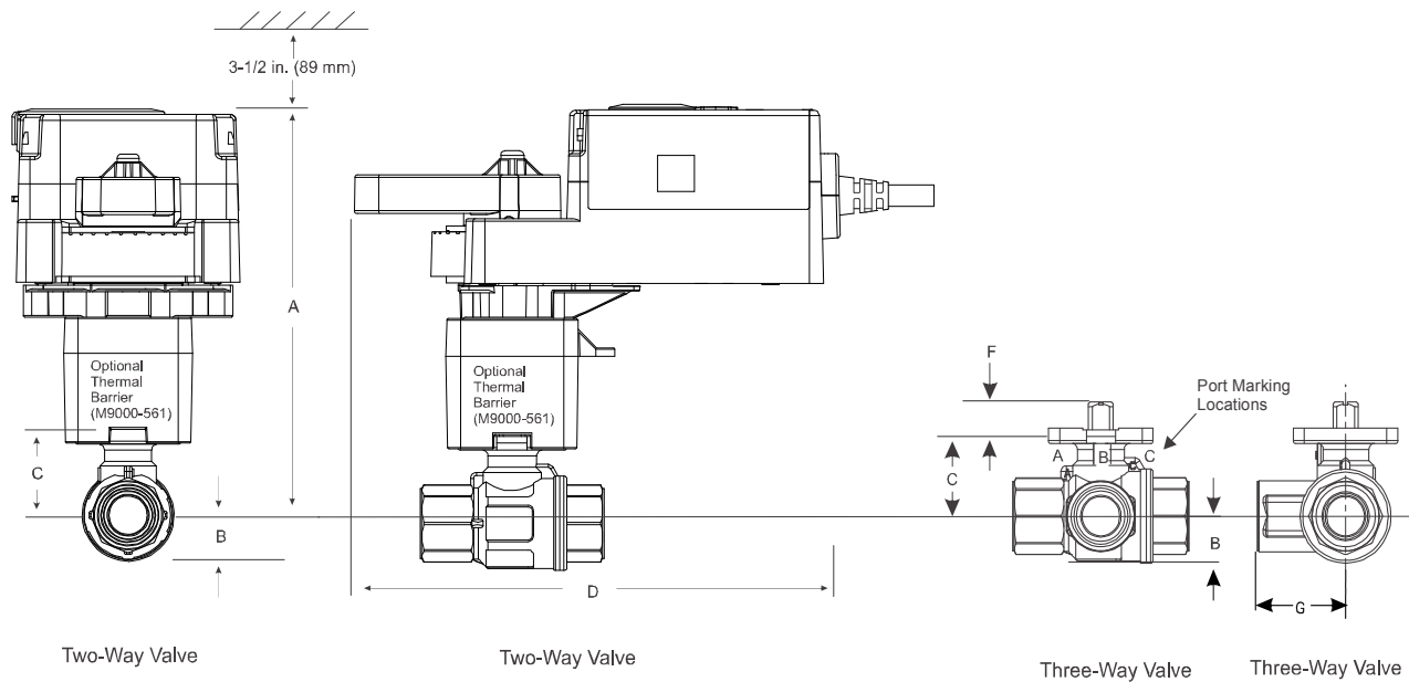
VA9300 Series Electric Non-Spring Return Actuator and Valve Dimensions (with Optional M9000-561 Thermal Barrier)
