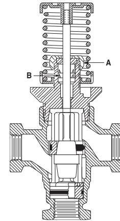
Repair Parts, V-4324 and VB-4324
