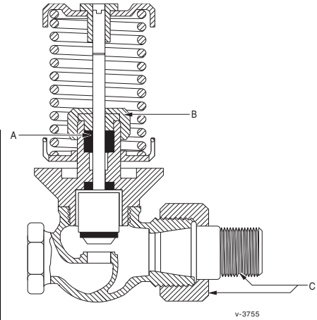
Repair Parts, V-3755
