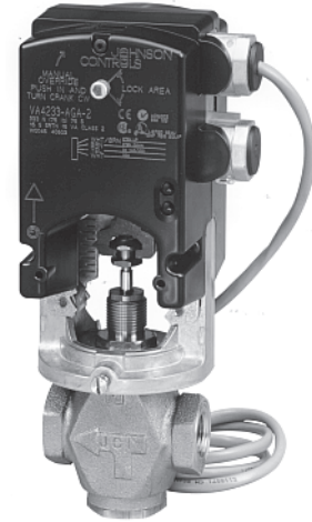
VA-4233 Series Electric Valve Actuator Mounted on a VG7000 Series Bronze Control Valve
