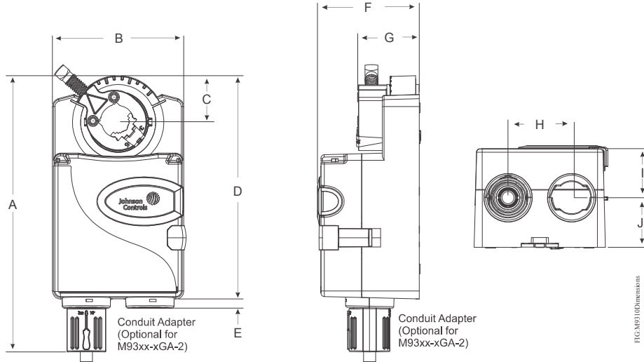
M9308 and M9310 Series Electric Damper Actuators, Dimensions (without Switch Kit or Potentiometer Kit)
