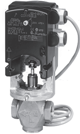
VA-4233 Electric Actuator Mounted on a VG7441 Brass Globe Valve
