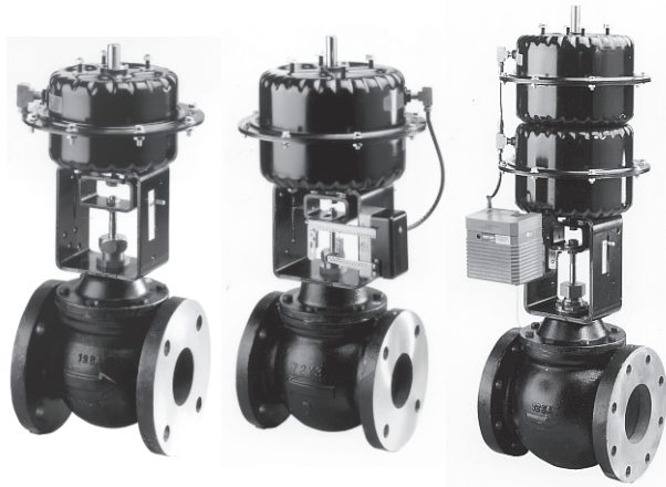
MP8000 Series Actuators Mounted on VG2231 Two-Way Normally Open Valves
