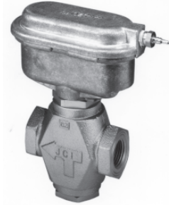
V-3801-8001 Pneumatic Actuator Mounted on VG7842 Brass Globe Valve
