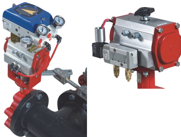
V-9000 Series Rotary Motion Rack and Pinion Pneumatic Actuators for Butterfly Valves
