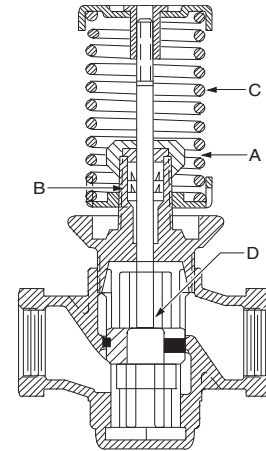
Repair Parts, V-3974 and VB-3974
