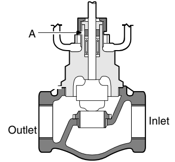
Repair Parts, V-7216
