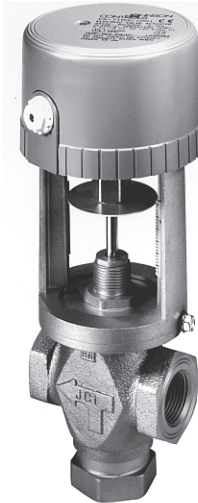
VA-715x Series Electric Actuator Mounted on a VG7842 Brass Globe Valve
