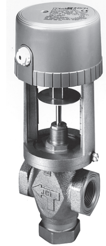
VA-715x Series Electric Actuator Mounted on VG7844 Brass Globe Valve
