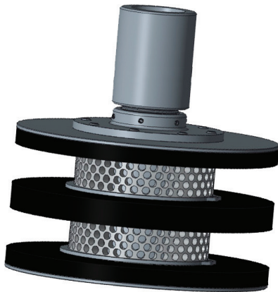
Figure 8: Acoustic Nozzle Exterior View
